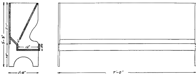
PLATE 24. Feed trough used at the University of Wisconsin, in which hay is fed to young lambs, and both hay and grain to older sheep.
